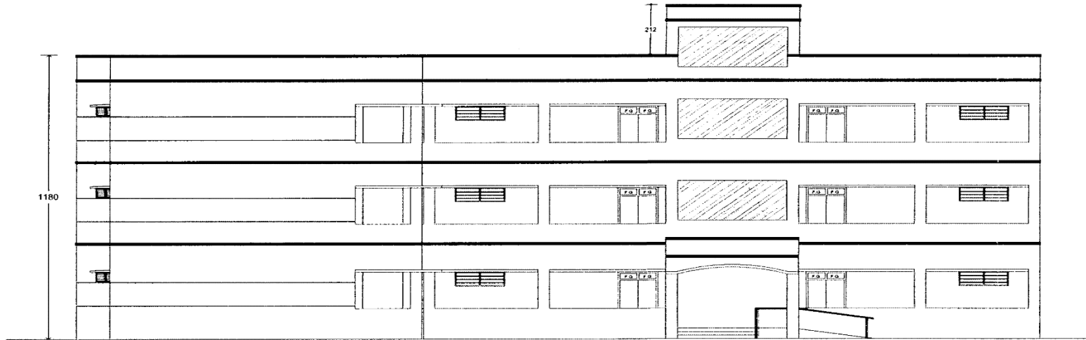
FRONT ELEVATION
